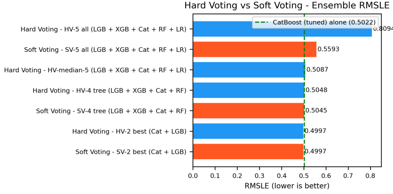
Figure 11: Hard Voting Vs Soft Voting
