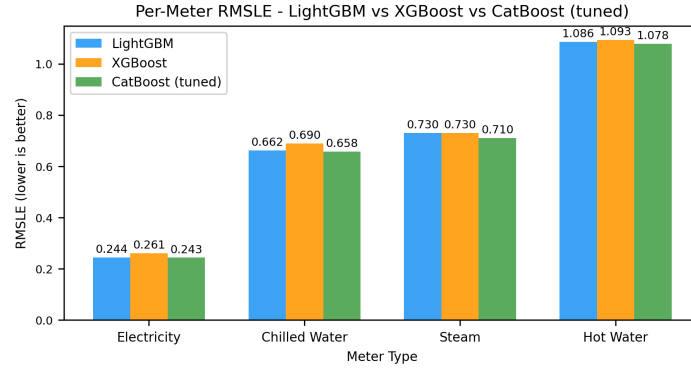
Figure 9: Per Meter RMSLE of the Boosting Models
